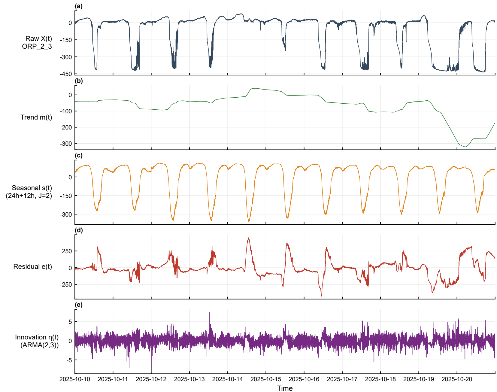
Multi-scale decomposition — ORP_2_3 (pre_anoxic_rear, min) [2025-10-10~2025-10-20]
